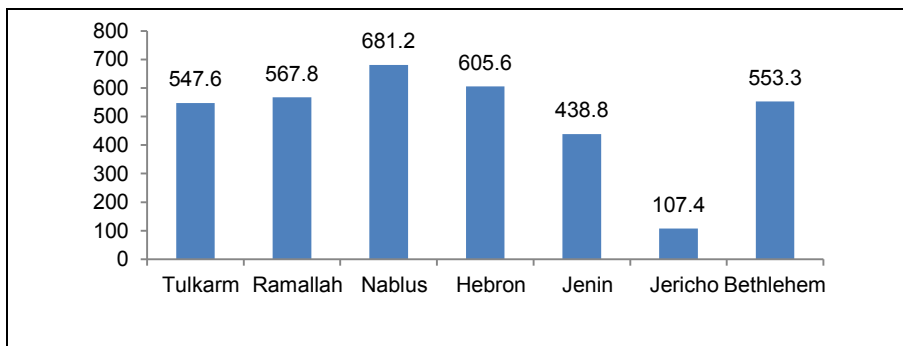
Annual Rainfall Quantity(mm) in the West Bank by Station Location, 2016
